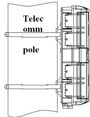
Pic 5 Pole ring installation
