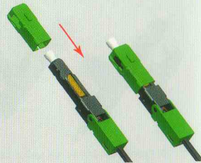
10. Install the housing and complete the assembly.
