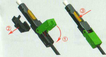
9. Press the cover to lock drop cable, then remove the opener, finally press the box shell, locking bare fiber.
