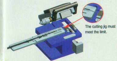
5. Use the cutting jig to cut the bare fiber.
