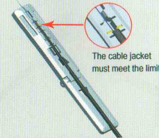
4. Put the cable in the cutting jig to fix.
