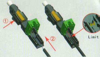
7. Press the opener to right position, then insert fiber from connector tail till limit.
