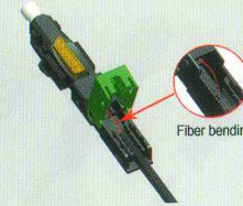
8. Check whether the rear fiber is bent, if not, re-cut the fiber and assembly.
