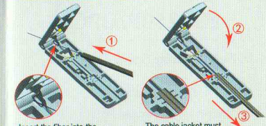
Insert the fiber into the guide port of cylindrical pin.
