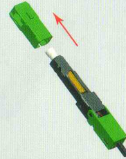
①. Hold on the dust cap and remove the housing.
