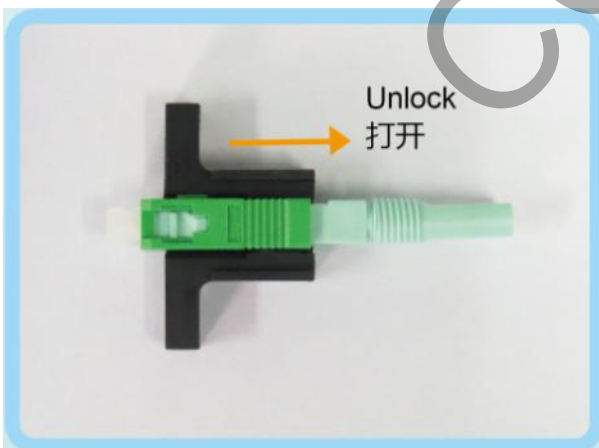
2.1 Check the locker
