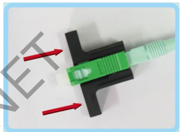
3.2 Unlock the fiber
