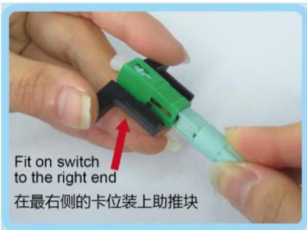
3.1 Assemble the auxiliary jig
