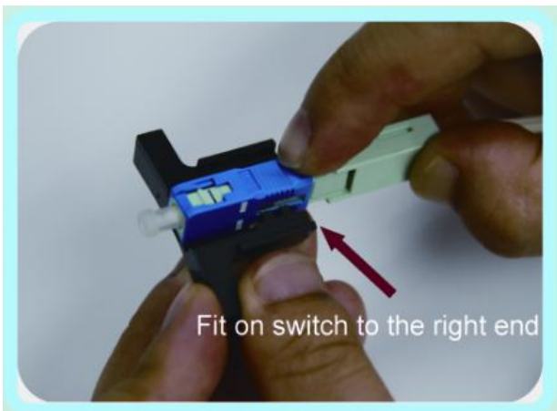
3.1 Assemble the auxiliary jig
