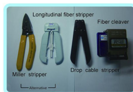
3. Recommended Installation tools
