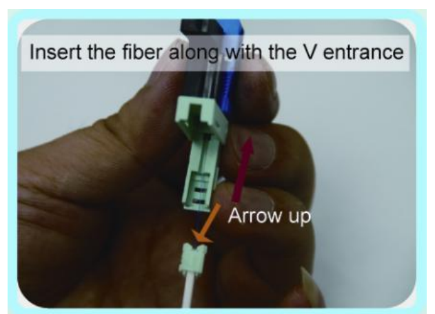
2.2 Insert the fiber
