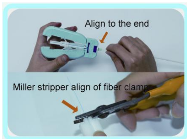
1.3 Strip the cable coating layer
