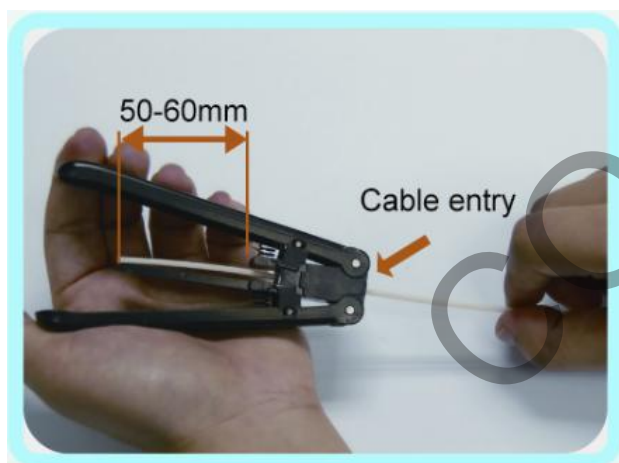
1.1 Strip the cable strengthen layer
