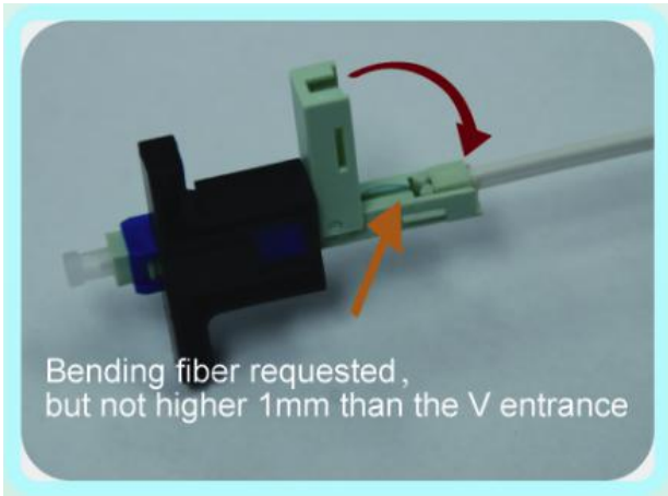
2.3 Complete the fiber insertion
